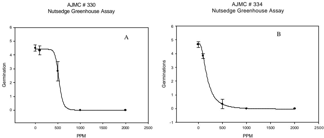
Figure 2. Nutsedge Greenhouse Assay. A. AJMC # 330. y=4.42/(1+(x/525)^{11.53}) Adj R^2 = 0.84 B. AJMC # 334. y=(4.6666+0.0040x)/(1+0.0021x) Adj R^2 = 0.95 .
